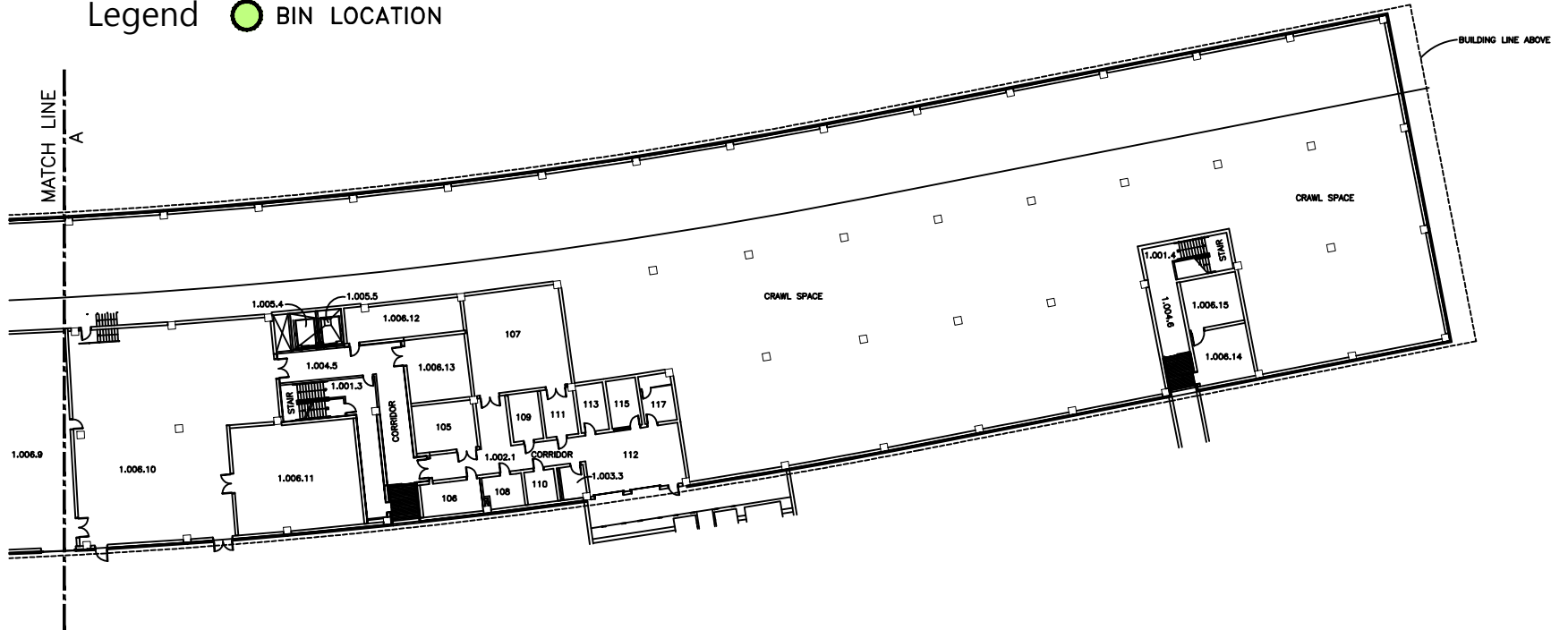
1st Level Floor Plan East
